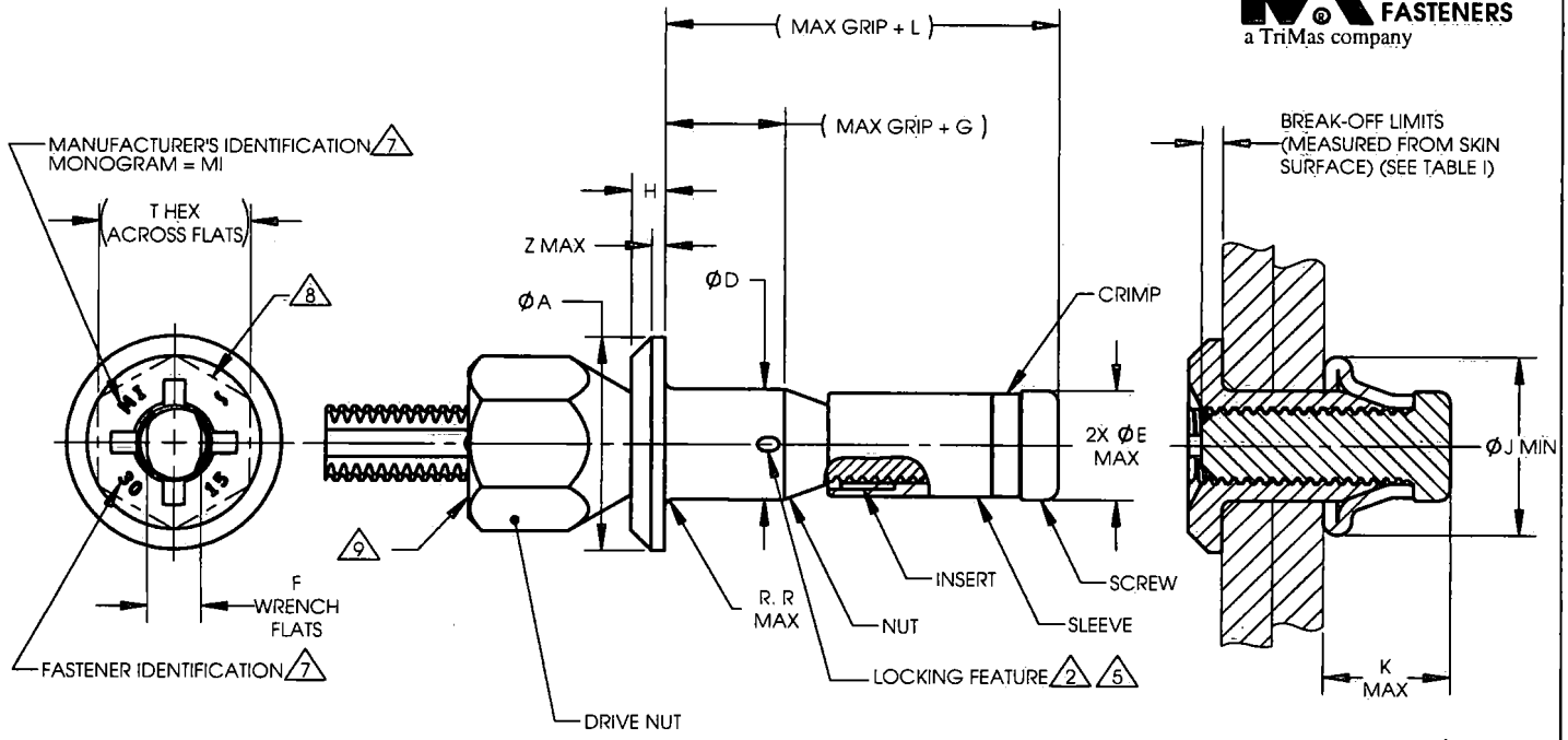
TYPICAL INSTALLATION 6
